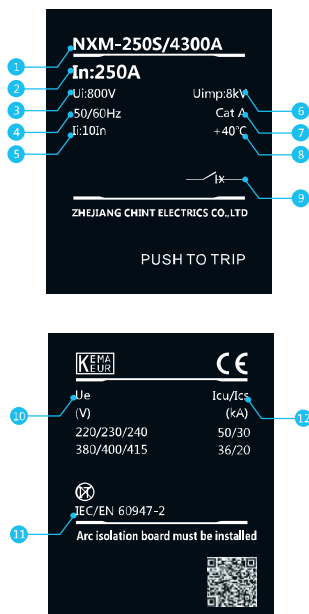
NXM Nameplate of thermomagnetic stationary molded case circuit breaker
