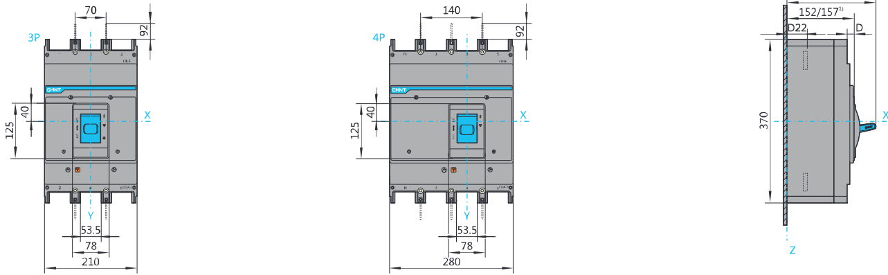
Front connection, dimension (mm)
