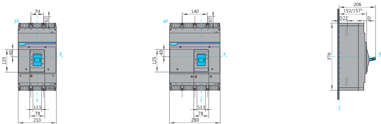
Front connection, dimension (mm)
